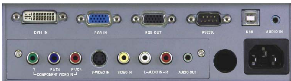
Input/Output Terminals
